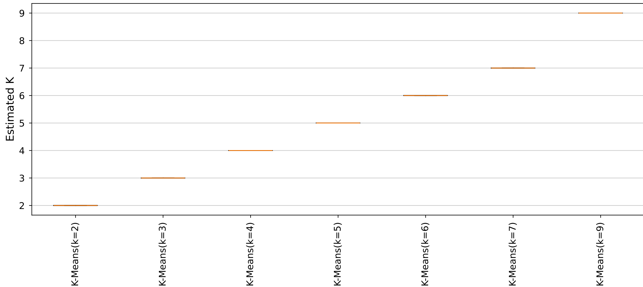
YARA Rules Estimated K Distribution (Cluster11_Size9 dataset)
